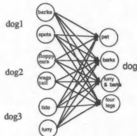
Figure 1 (Hanson). The four possible kinds of representational relations between tokens and types. On the left are two kinds of hidden-layer localist representations. On the right are two kinds of distributed representation.
