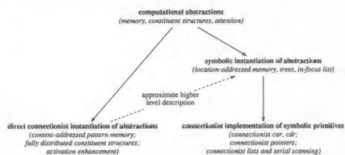
Figure 1. The methodological implications of limitivist (left branch) vs. implementationalist (right branch) views of connectionism.
